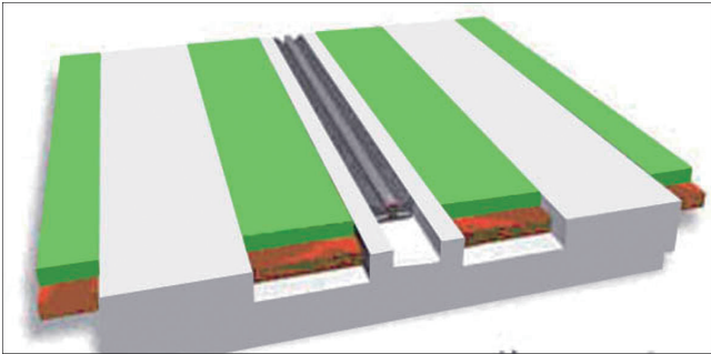
图 4 胶轮+导轨式现代有轨电路面结构 Fig.4 Road structure of rubber-tyred trams
