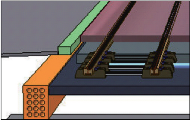
图3 钢轮钢轨式现代有轨电车路面结构 Fig.3 Road structure of steel-wheeled trams
